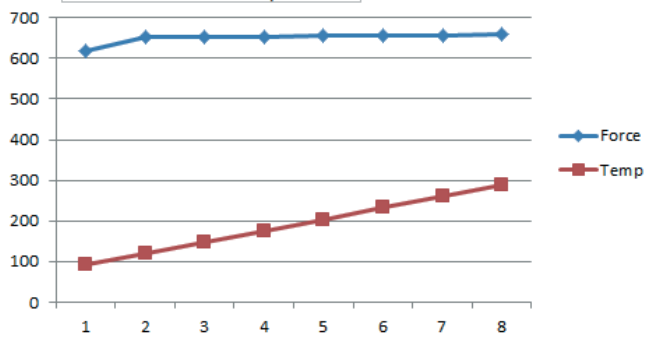
First Fade Force vs Temp
