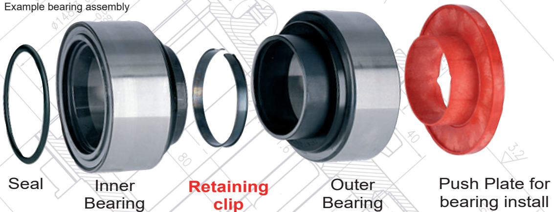
Example bearing assembly
